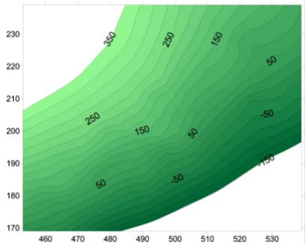
Figure 2 Contour map of the Sub-Upper Chalk surface made by universal kriging. Units are meters, the co-ordinates are in kilometers.
