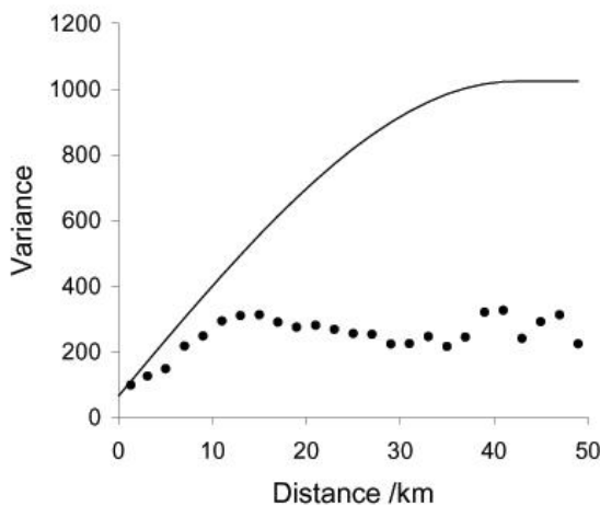
Figure 1 Variograms of height of Sub-Upper Chalk surface. The black discs form the experimental variogram of the residuals from the quadratic surface fitted to the data by ordinary least squares regression, the continuous line is the variogram estimated by REML.
